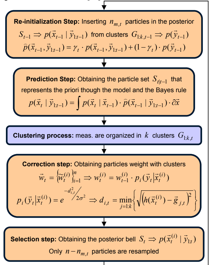
Fig. 3. XPFCP Flowchart
