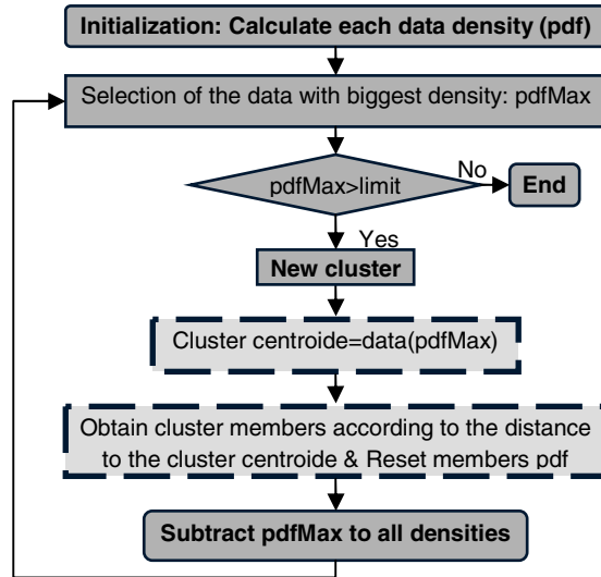
Fig. 3. Flowchart of the modified ‘Subtractive’ algorithm proposed by the authors. Dashed lines remark the main improvements included in the standard version of the algorithm.
